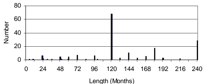
IDSi: Distribution of Max Sentences
